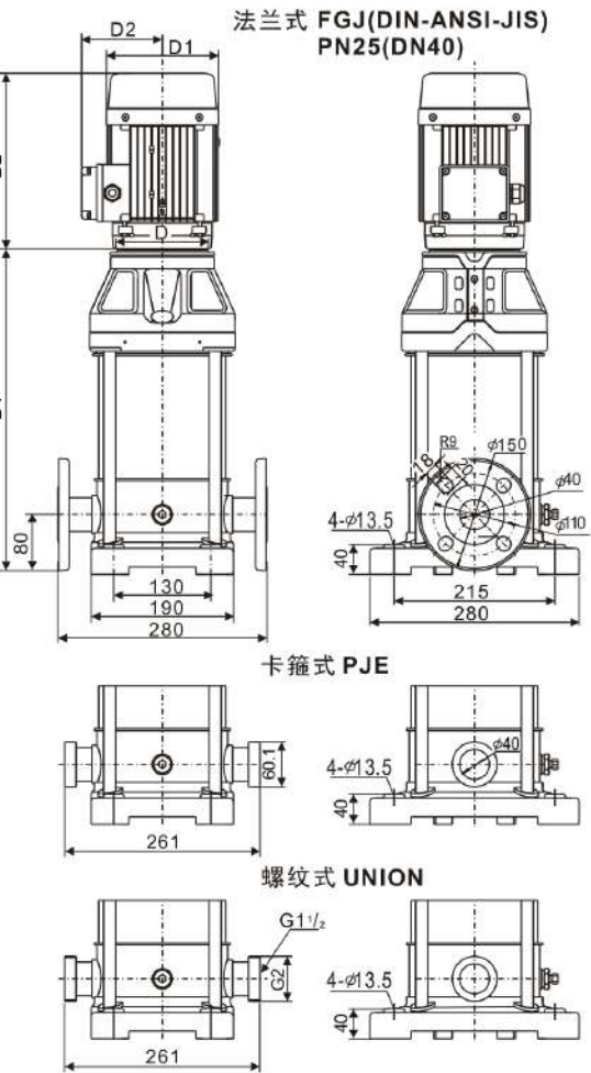
安装图/Installation sketch
