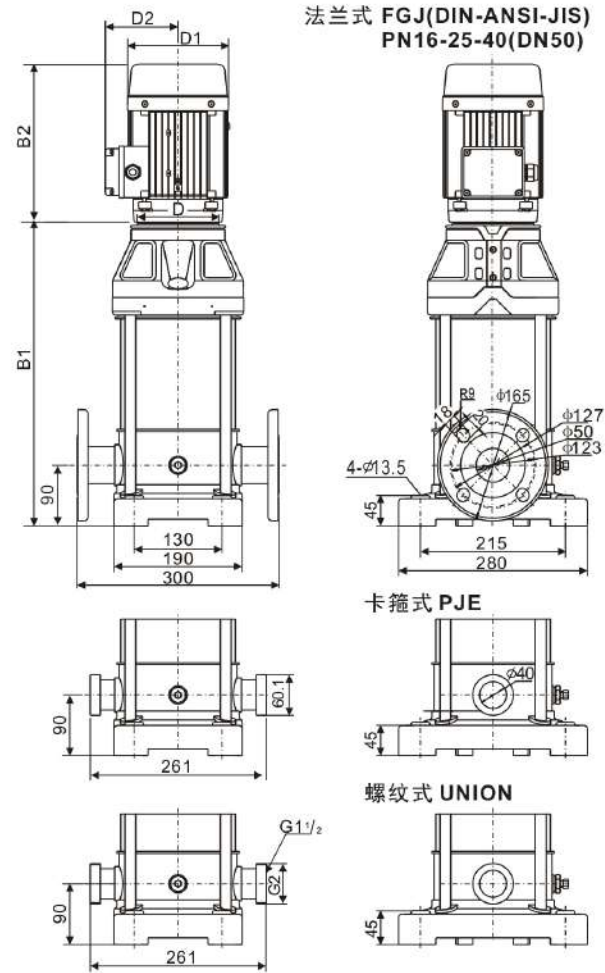
安装图/Installation sketch
